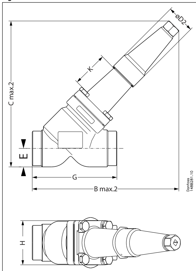
Figure 25: SVA-xx x x STR CAP
