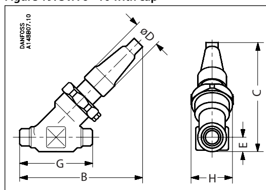
Figure 19: SVA 6 - 10 with cap
