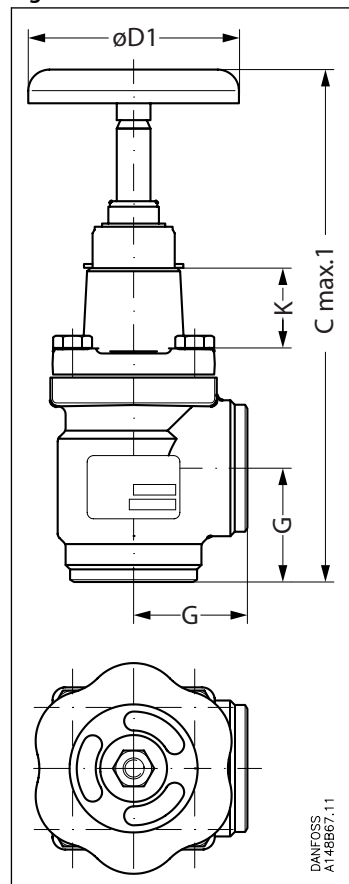
Figure 24: SVA-xx x x ANG H-WHEEL
