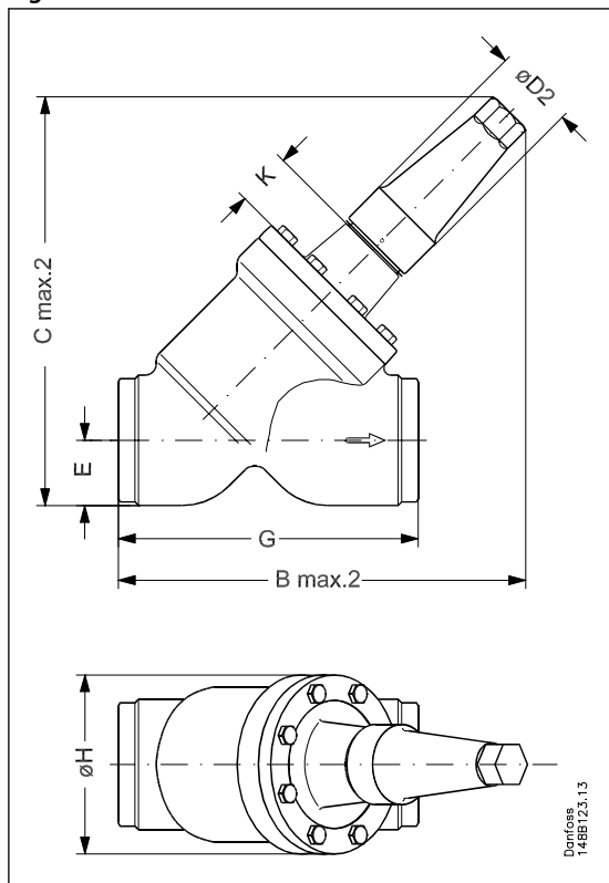
Figure 29: SVA-xx x x STR CAP
