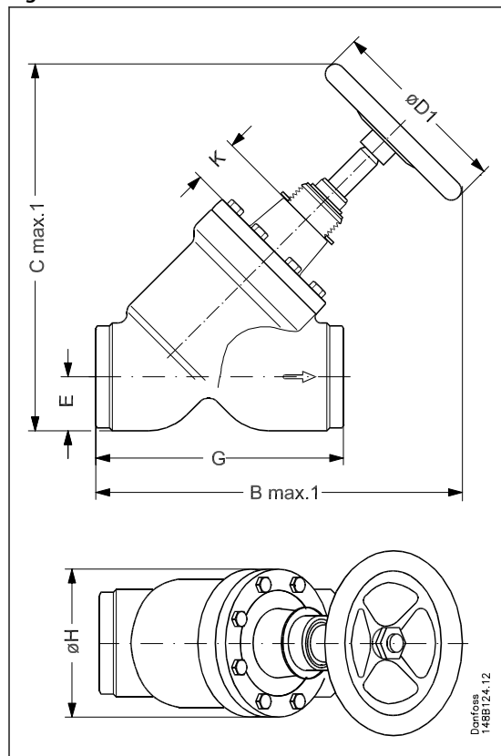
Figure 30: SVA-xx x x STR H-WHEEL
