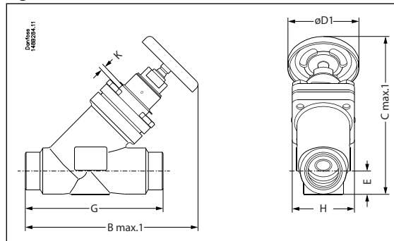
Figure 22: SVA-xx x x STR H-WHEEL
