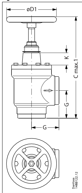
Figure 28: SVA-xx x x ANG H-WHEEL
