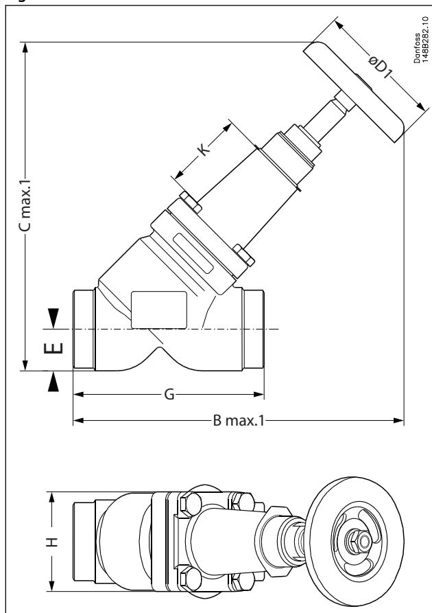
Figure 26: SVA-xx x x STR H-WHEEL
